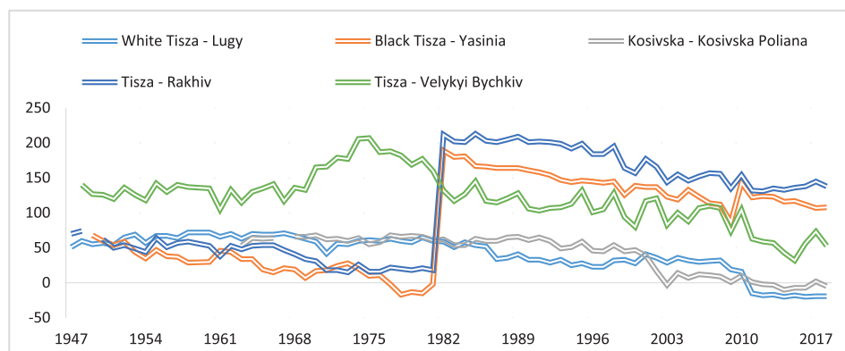
Fig. 1.2.2. Dynamics of water levels by annual averages, cm (compiled by the Zakarpattia Regional Hydrometeorological Centre)
