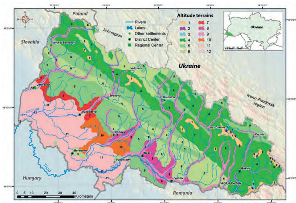
Fig. 1.8.2. Landscape map of Zakarpattia Region on the level of high-altitude terrains (based on the materials of A. Melnyk (1999) and M. Karabiniuk (2020)). Names of high-altitude terrains according to A. Melnyk (1999)
